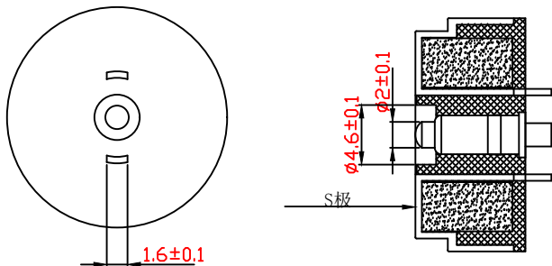
磁吸公头
