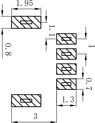
PCB LAYOUT
