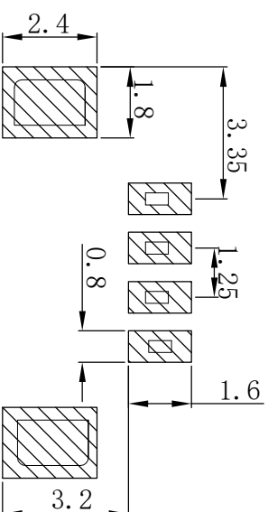
PCB LAYOUT
