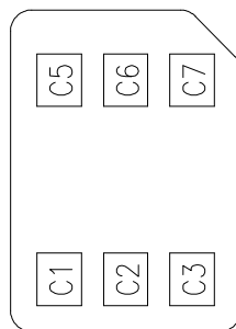
NANO SIM CARD PAD
