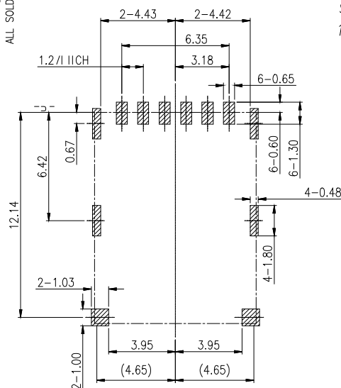
RECOMMENDED P.C.B. LAYOUT TOLERANCE (TOP VIEW) \pm 0.05\text{mm}
