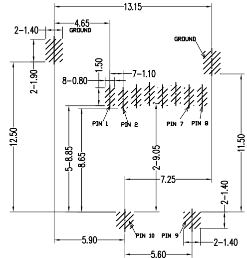
RECOMMENDED PCB LAYOUT (ALL TOLERANCE ARE \pm 0.05 )
